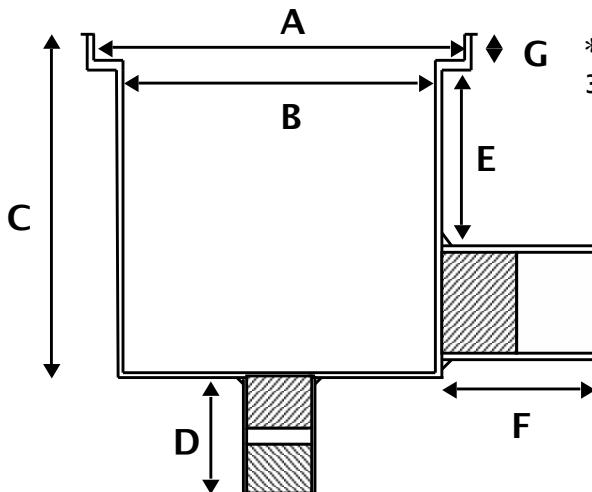
High Capacity Heavy Duty Fiberglass Sump Dimensions
