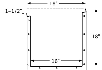
Zero Entry 18" Gutter
