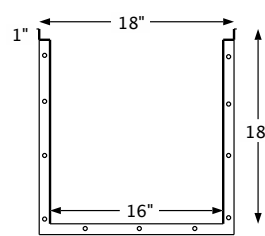
Level Top 18" Gutter
