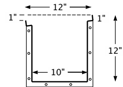
Zero Entry 12" Gutter
