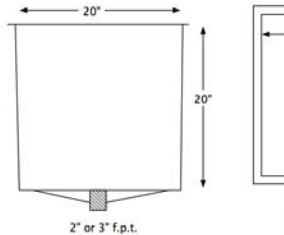
34 gallon Precoat Pot with 2" - part # fpk-70-101 with 3" - part # fpk-70-102
