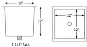
6 gallon Precoat Pot part # fpk-70-100
